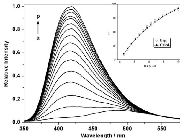
Figure 2. Fluorescence spectral changes of 1 ( 1.0 \times 10^{-5} M) upon addition of \text{Cd}(\text{ClO}_4)_2 ( 0\text{--}1.2 \times 10^{-2} M, from a to p) in HEPES buffer solution (10 mM, pH 7.2). Inset: The nonlinear least-squares analysis of the differential intensity ( \Delta F ) to calculate the complex formation constant ( K_s ). ( \lambda_{\text{ex}} = 303 nm, \lambda_{\text{em}} = 418 nm).
