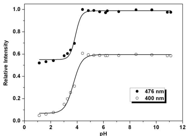
Figure 1. Plot of fluorescence intensity at 400 and 476 nm of 1 versus pH value in aqueous solution. ( [\mathbf{1}] = 2.0 \times 10^{-5} M, \lambda_{\text{ex}} = 300 nm).
